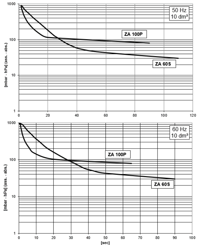
NOTE: Curves refers to 1013mbar (abs.) pression and 20°C temp. (tolerance ±10%).
